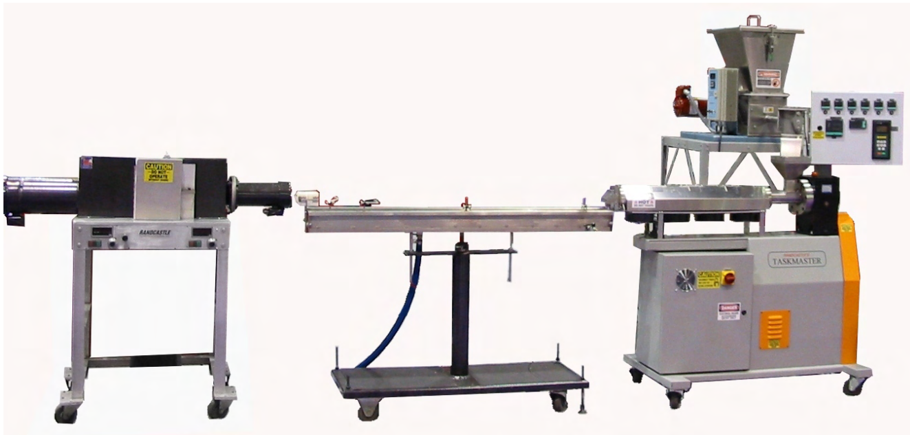
RCP-2.0 Pelletizer with dual drives
